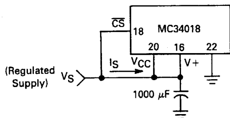
FIGURE 14 — ALTERNATE POWER SUPPLY CONFIGURATION
