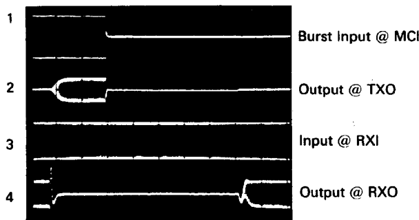
FIGURE 16 — TRANSMIT-RECEIVE SWITCHING
